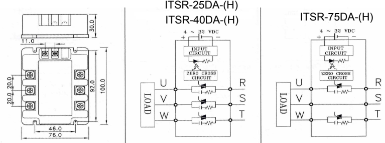
ITSR 3-Phase Solid State Relay Wiring Diagram
