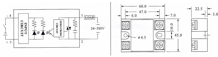
ISSR 1-Phase Solid State Relay Wiring Diagram
