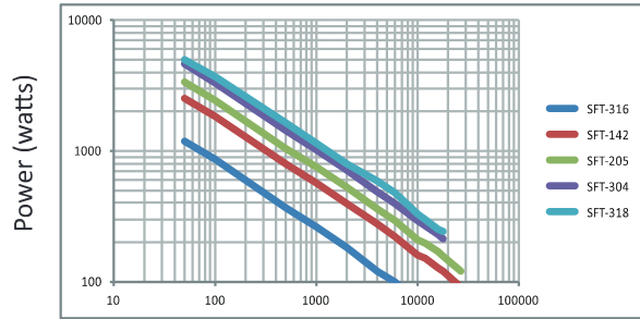
Power Handling vs. Frequency (Maximum)
