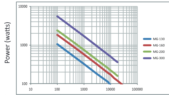
Power Handling vs. Frequency (Maximum)
