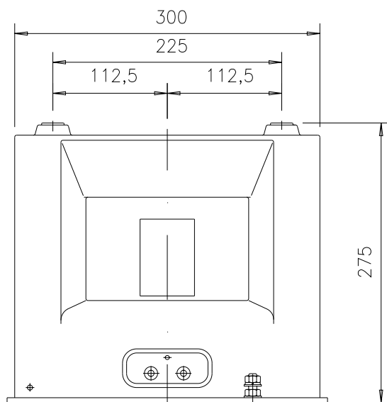
Bornes M6 Secondary terminals M6
