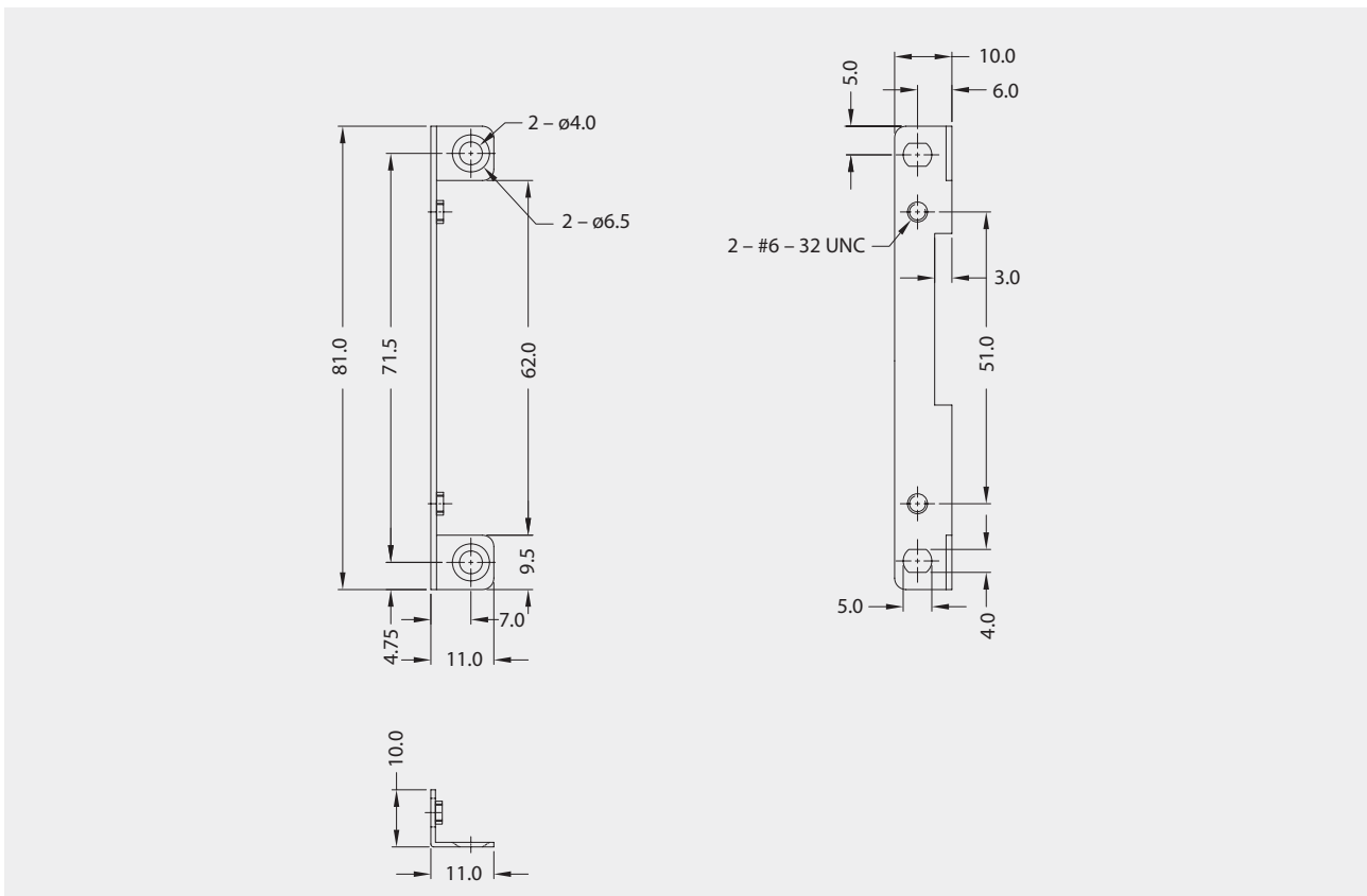
Mounting bracket included in delivery
