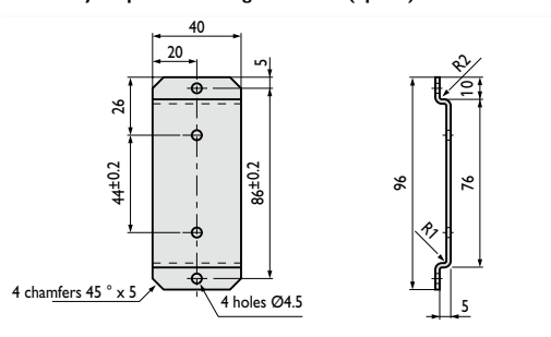
Accessory for plate mounting with screw (option)
