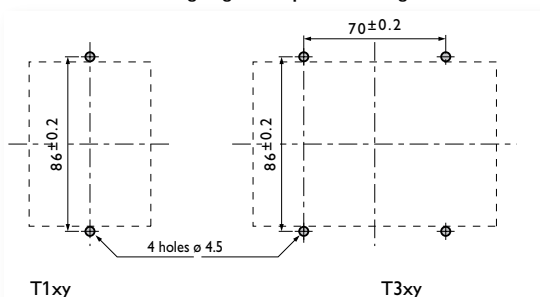
Panel drilling diagram for plate mounting
