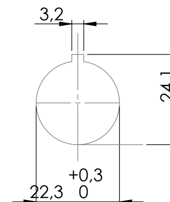
Bohrbild / Hole pattern
