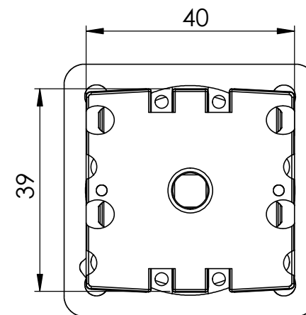
Bohrbild / Hole pattern
